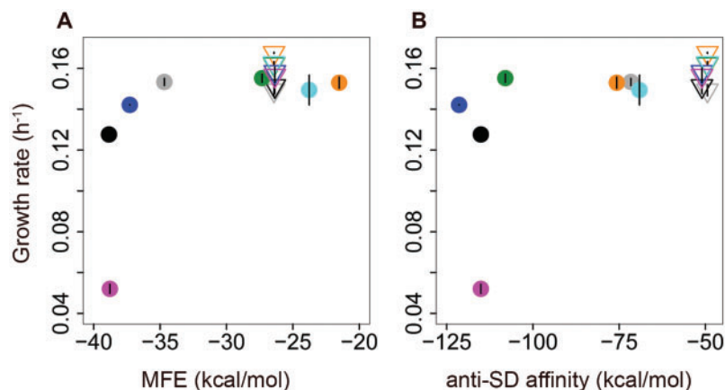
Fig. 4. Effect of N-terminal insert on fitness. Mean Growth rate ( \pm SEM; n = 3 biological replicates) of strains carrying plasmid-borne fae alleles induced with 1 \mu M cumate is shown as a function of (A) 5' MFE and (B) anti-SD affinity. Filled circles indicate ancestral fae alleles, and open inverted triangles indicate alleles carrying the N-terminal insert rich in frequent codons. Points are colored as in figure 1. For MFE calculations we used 100 bp long sequences ( -50 to +50 bp relative to the fae start site). For anti-SD affinity calculations, we used 55 bp long sequences ( -5 to +50 bp relative to the fae start site).
